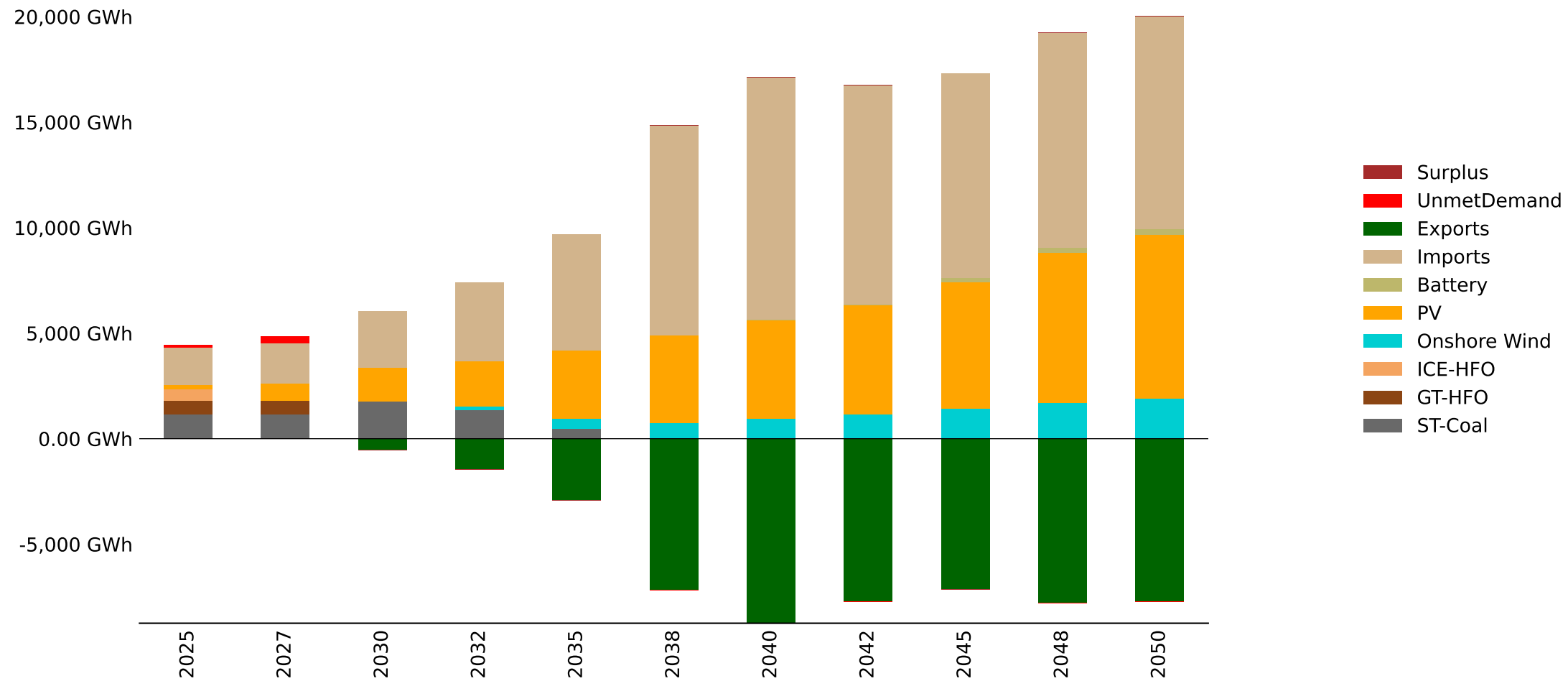
Energy Mix by Fuel - Botswana - baseline_INGA (GWh)
