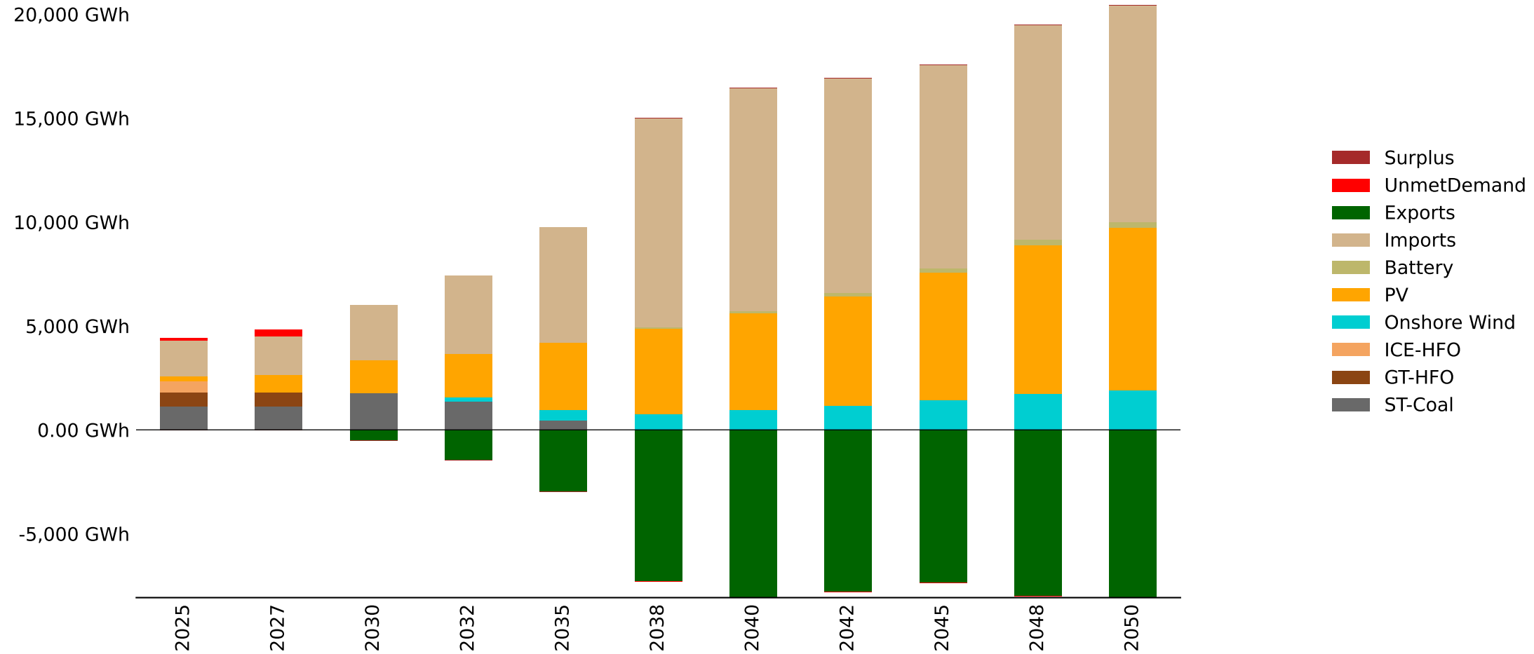
Energy Mix by Fuel - Botswana - baseline_noBTKG (GWh)
