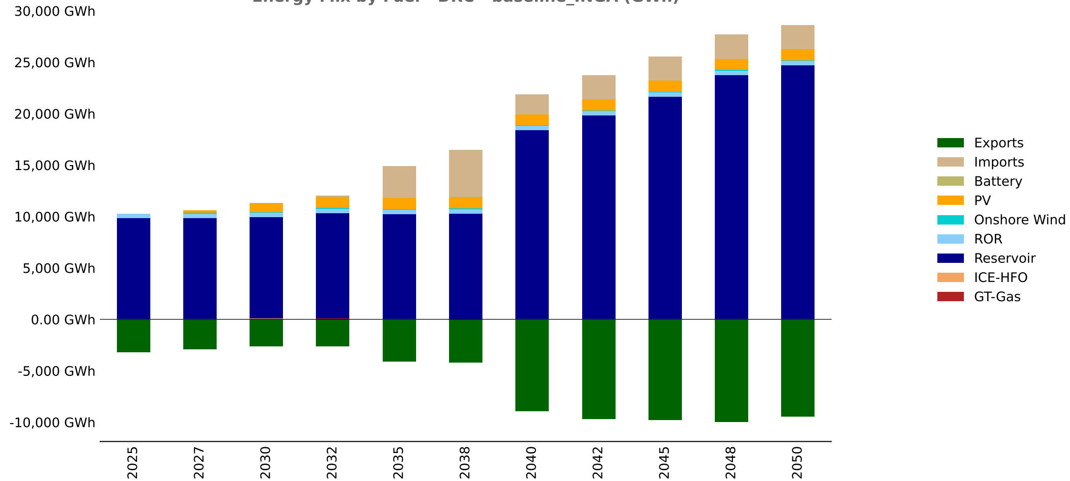
Energy Mix by Fuel - DRC - baseline_INGA (GWh)
