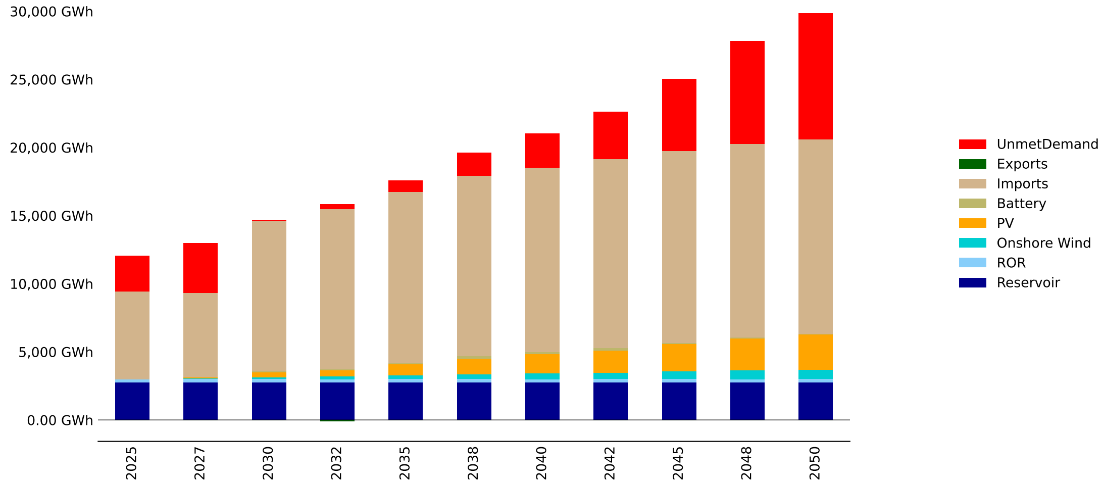
Energy Mix by Fuel - DRC_South - baseline_INGA (GWh)
