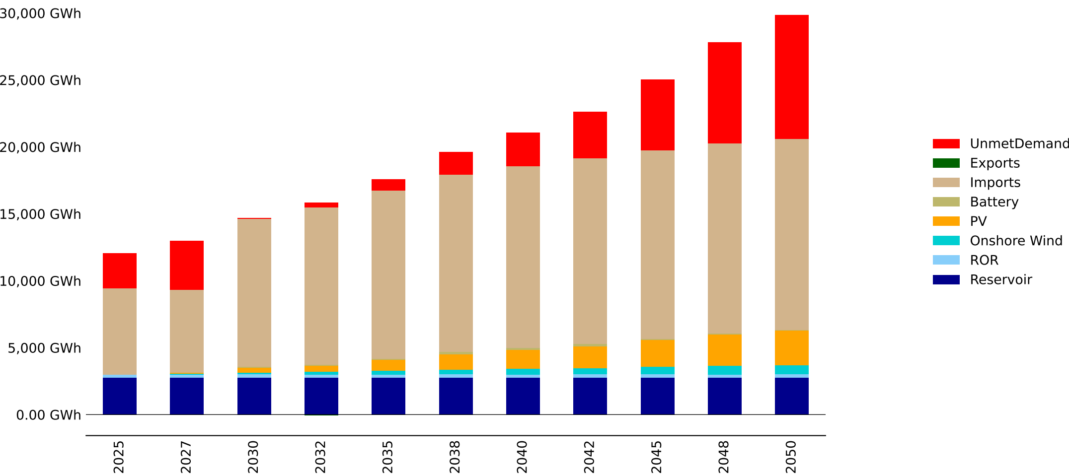
Energy Mix by Fuel - DRC_South - baseline_limexp (GWh)
