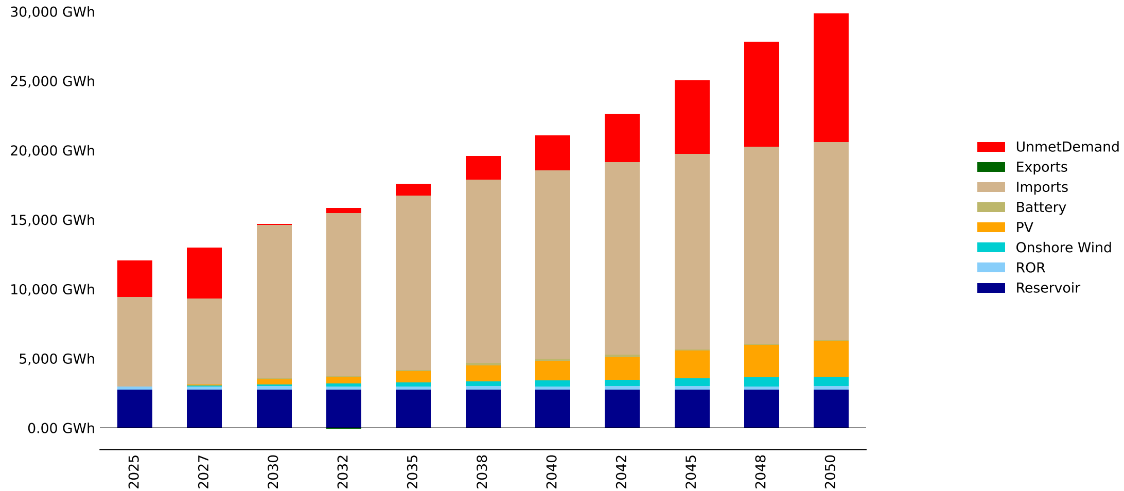
Energy Mix by Fuel - DRC_South - baseline_noBTKG (GWh)
