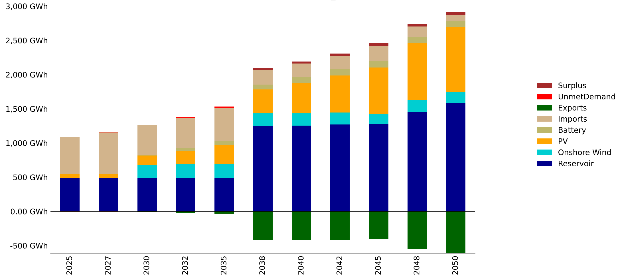
Energy Mix by Fuel - Lesotho - baseline_INGA (GWh)
