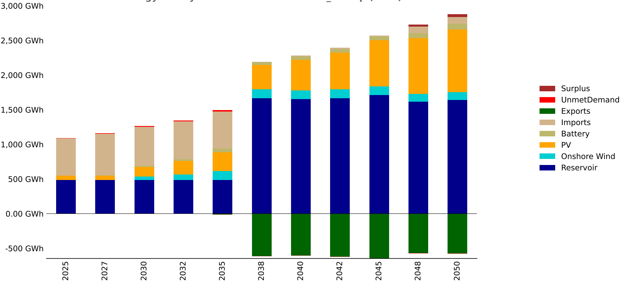
Energy Mix by Fuel - Lesotho - baseline_limexp (GWh)
