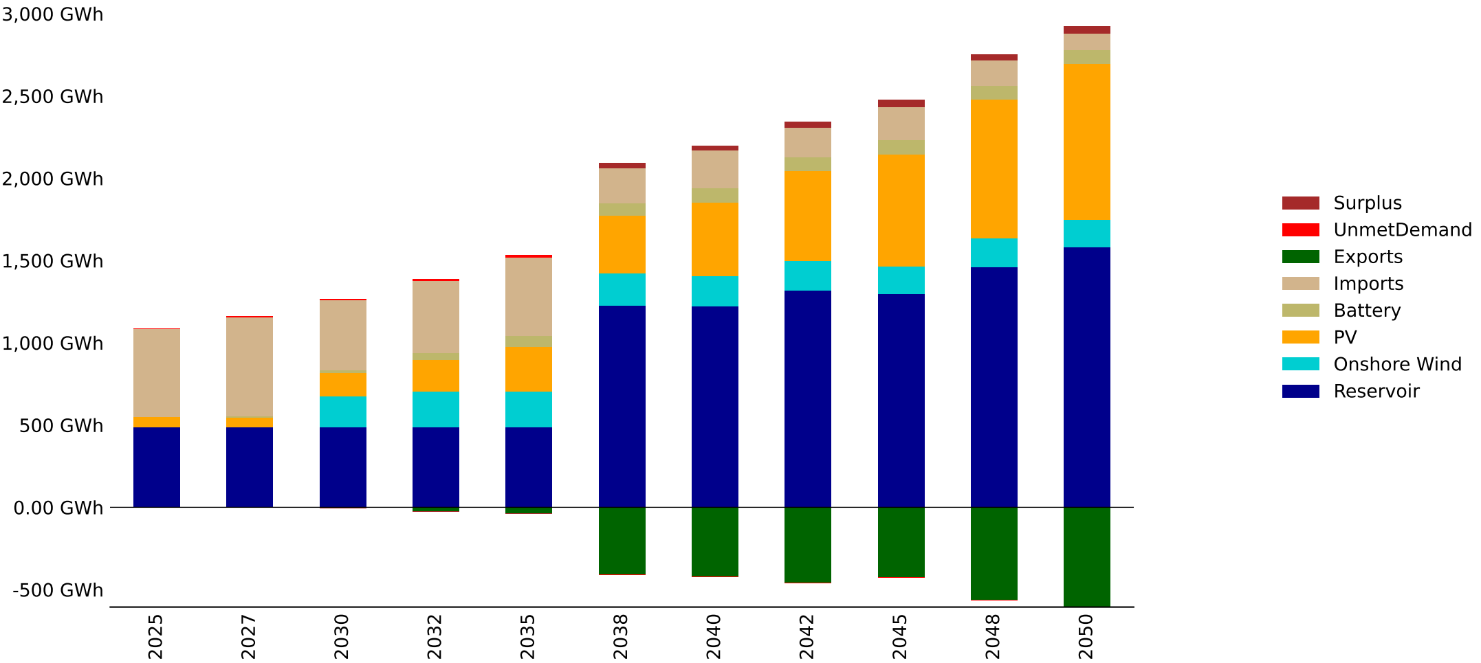
Energy Mix by Fuel - Lesotho - baseline_noBTKG (GWh)
