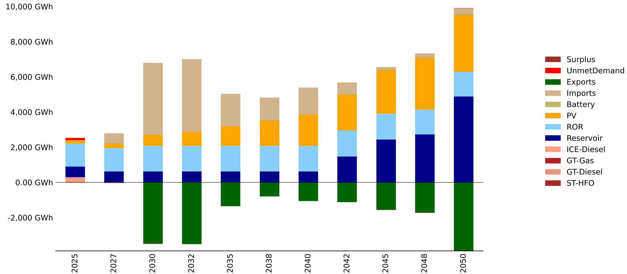
Energy Mix by Fuel - Malawi - baseline_noBTKG (GWh)
