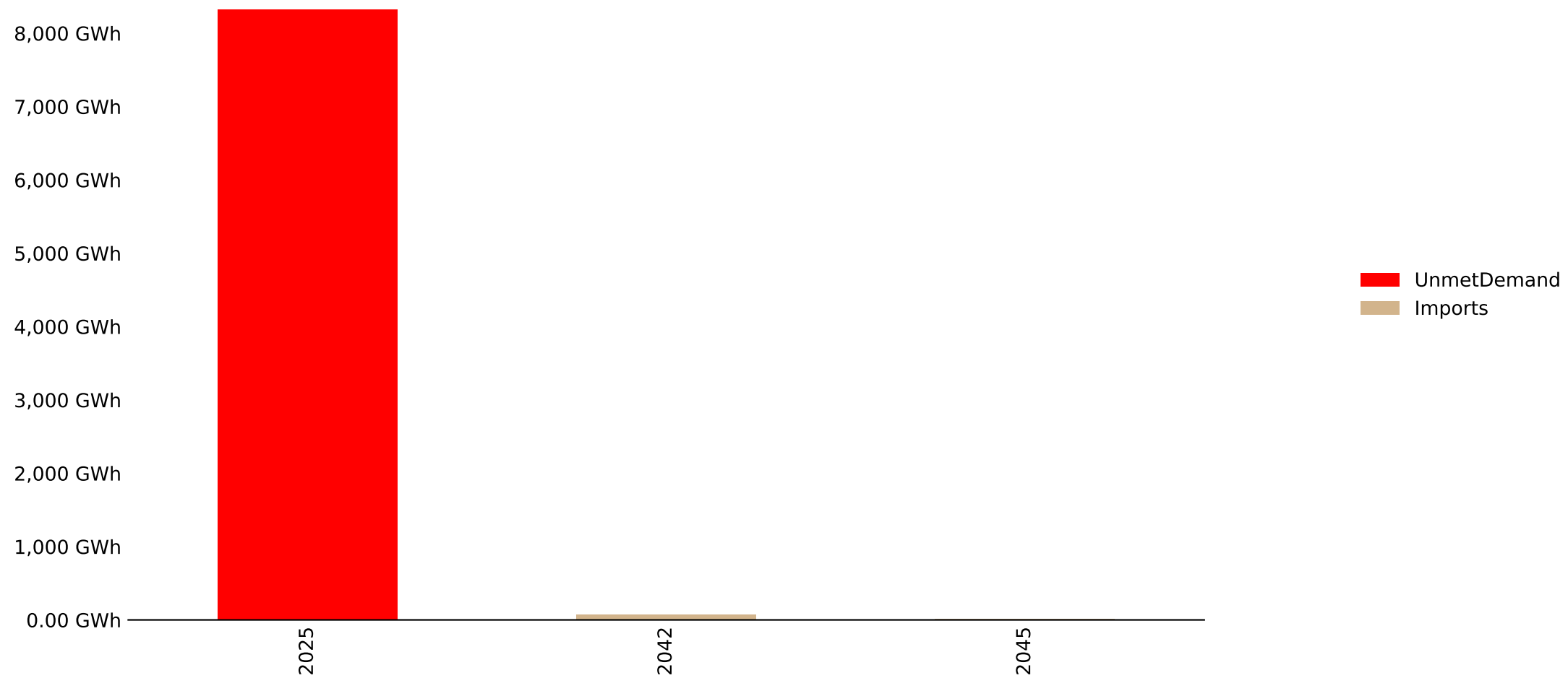
Energy Mix by Fuel - Mozal - baseline_INGA (GWh)
