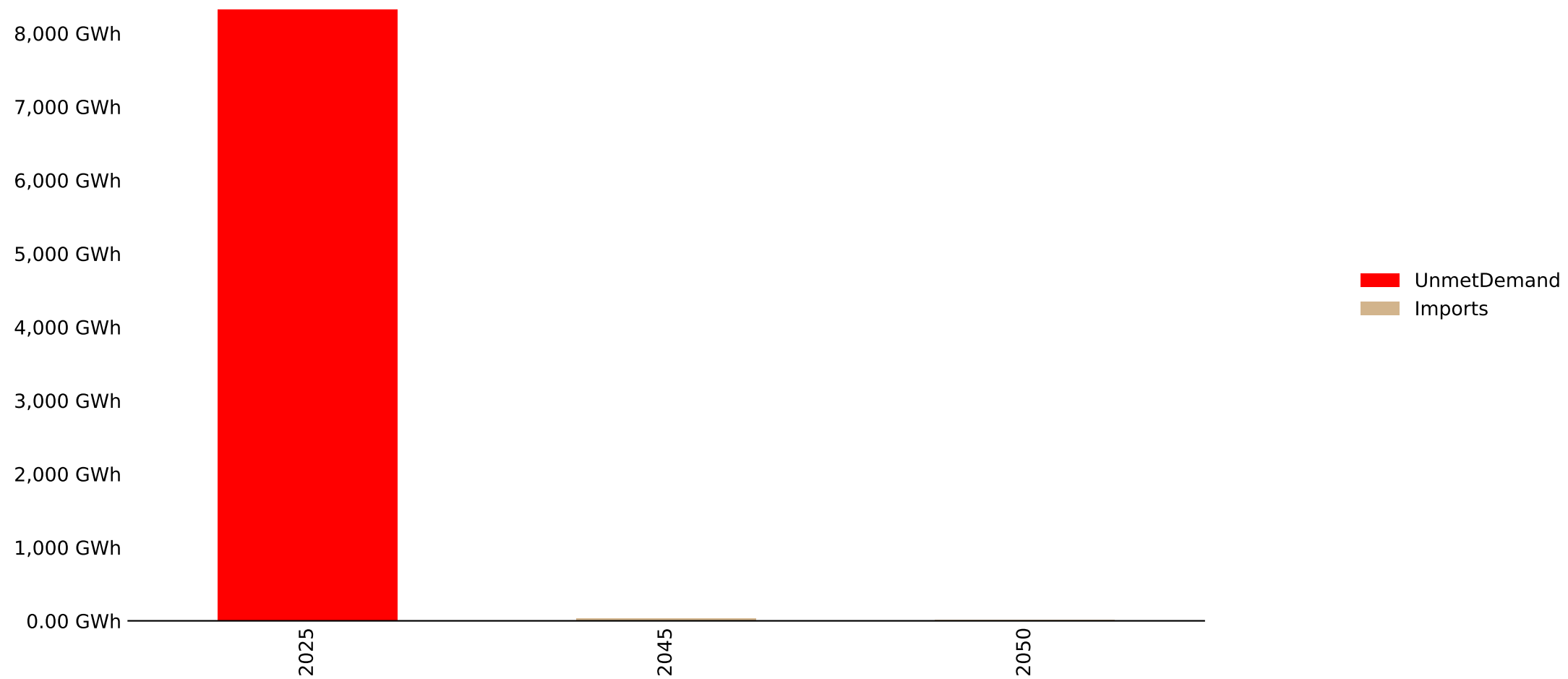
Energy Mix by Fuel - Mozal - baseline_noBTKG (GWh)
