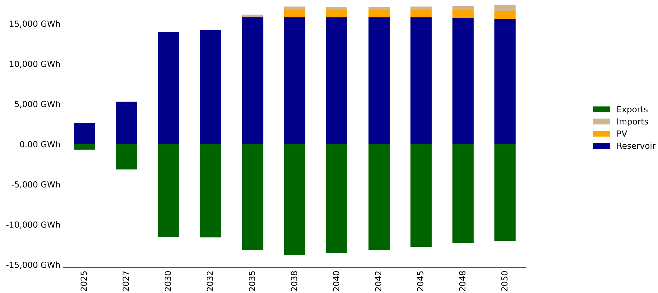
Energy Mix by Fuel - Mozambique_Central - baseline (GWh)
