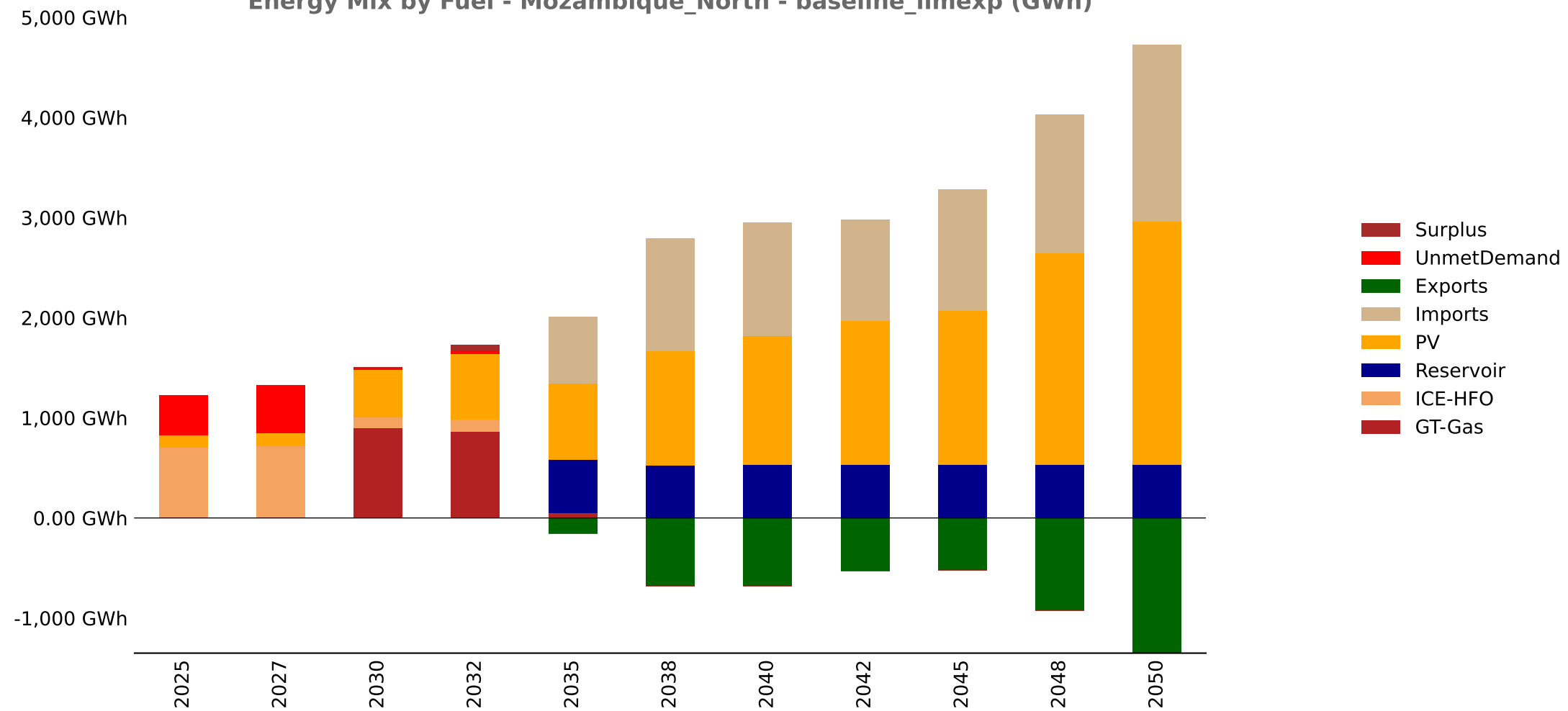
Energy Mix by Fuel - Mozambique_North - baseline_limexp (GWh)
