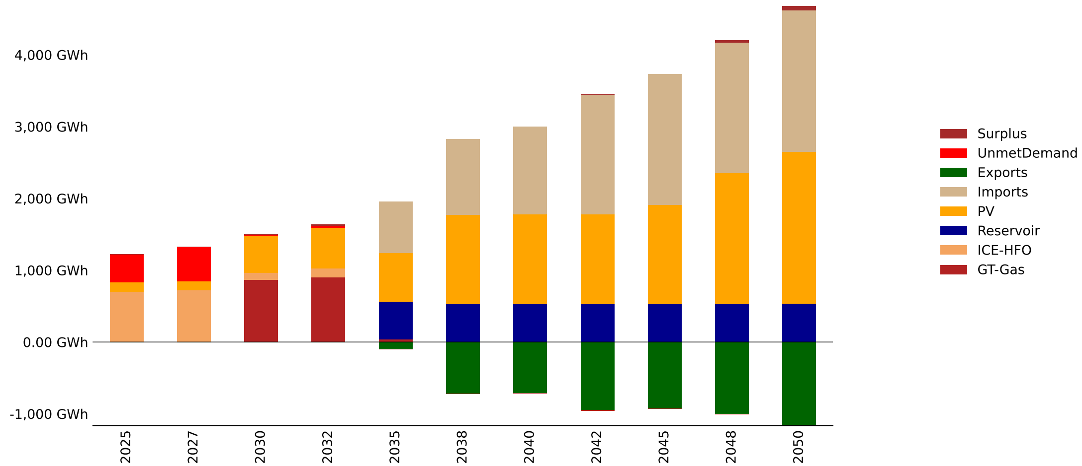
Energy Mix by Fuel - Mozambique_North - baseline_noBTKG (GWh)
