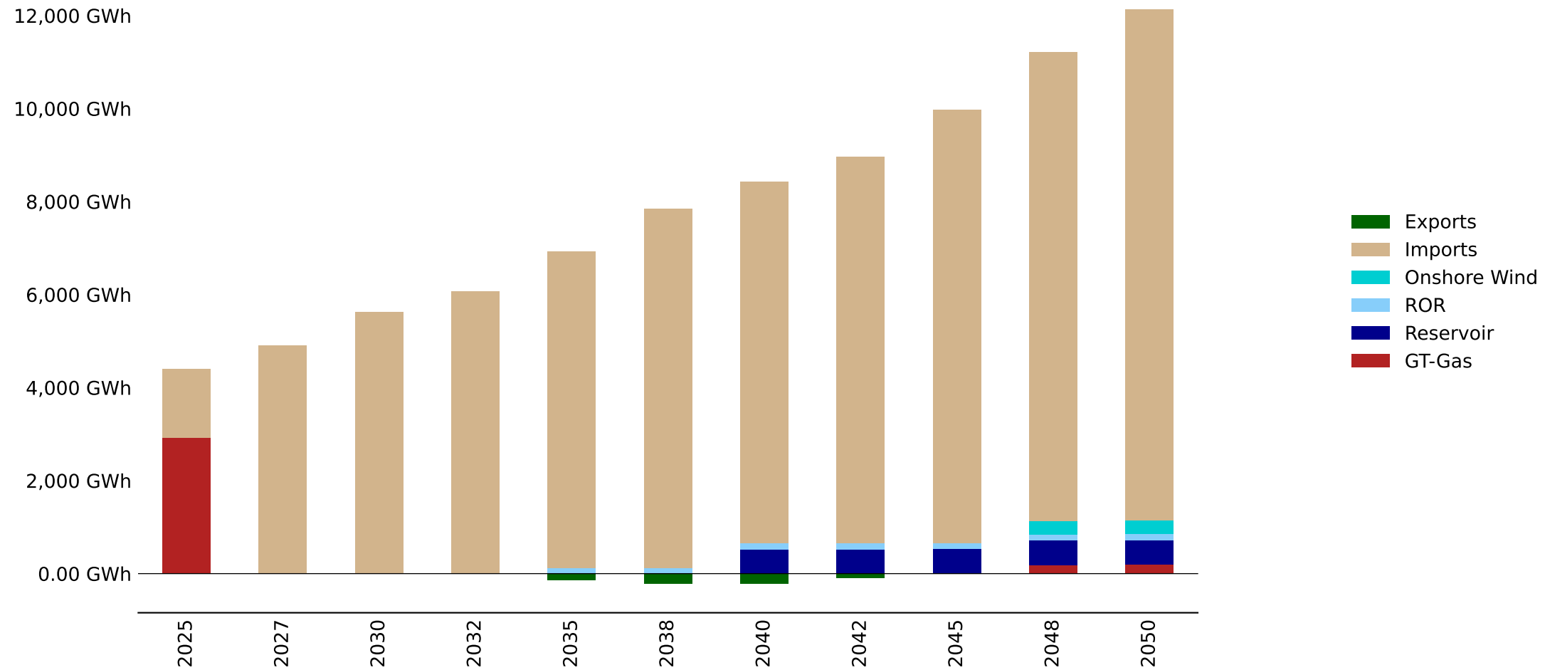
Energy Mix by Fuel - Mozambique_South - baseline (GWh)
