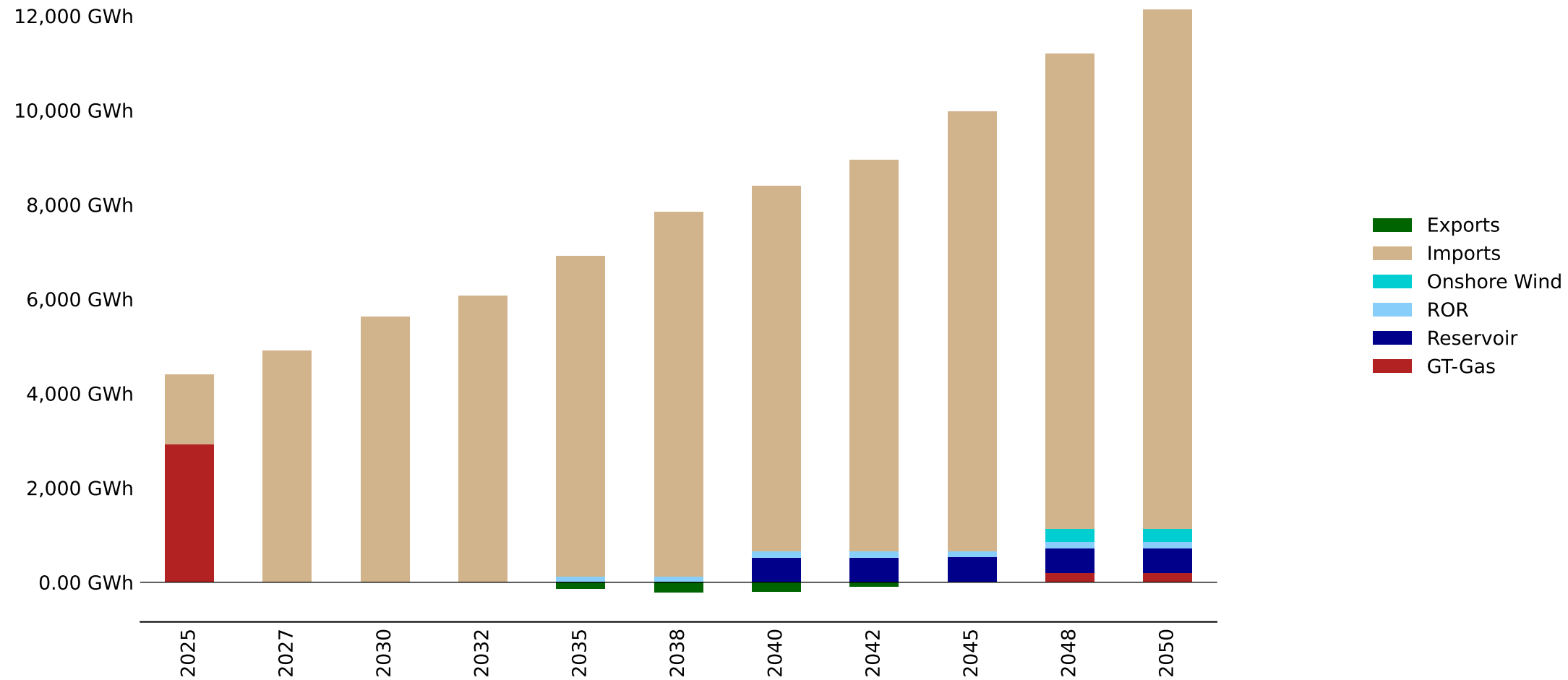
Energy Mix by Fuel - Mozambique_South - baseline_INGA (GWh)
