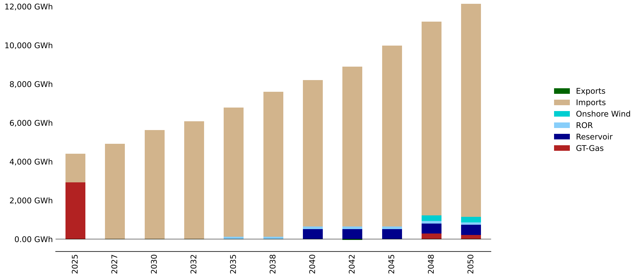
Energy Mix by Fuel - Mozambique_South - baseline_limexp (GWh)
