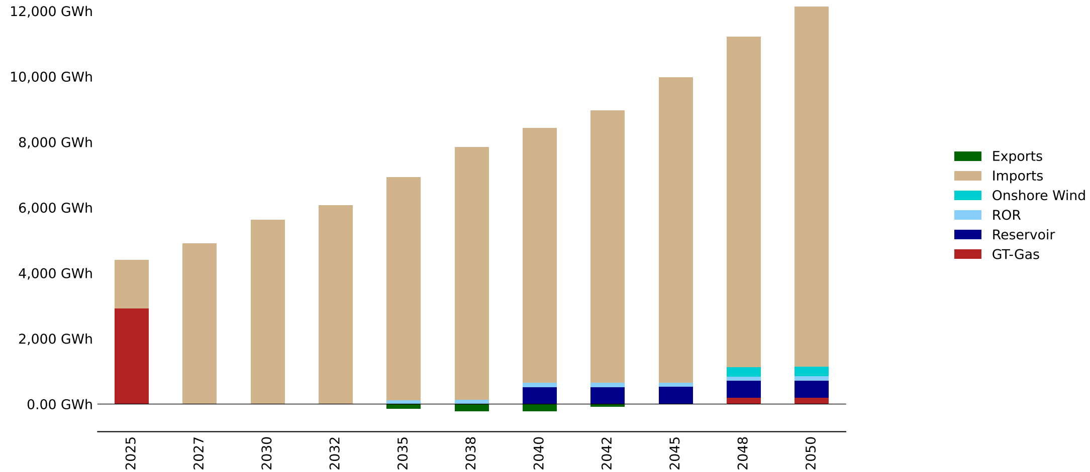
Energy Mix by Fuel - Mozambique_South - baseline_noBTKG (GWh)
