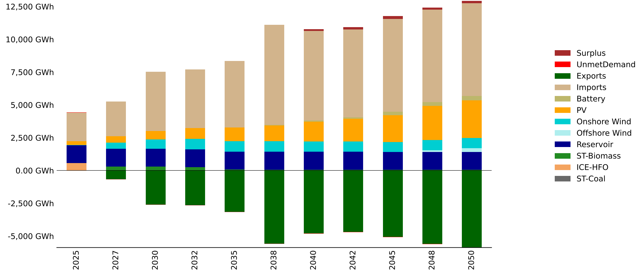
Energy Mix by Fuel - Namibia - baseline_INGA (GWh)
