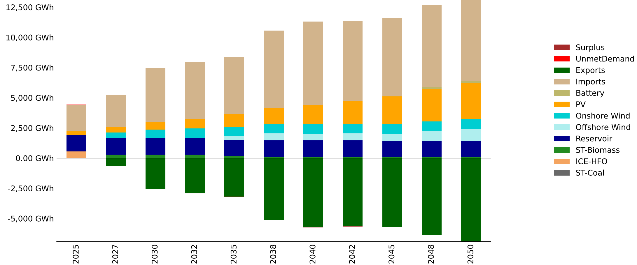
Energy Mix by Fuel - Namibia - baseline_limexp (GWh)
