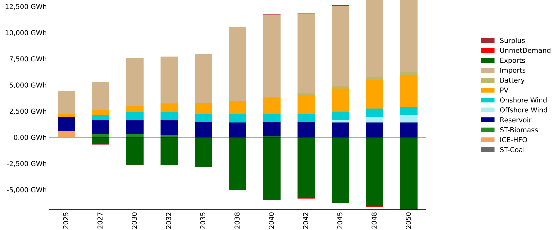
Energy Mix by Fuel - Namibia - baseline_noBTKG (GWh)
