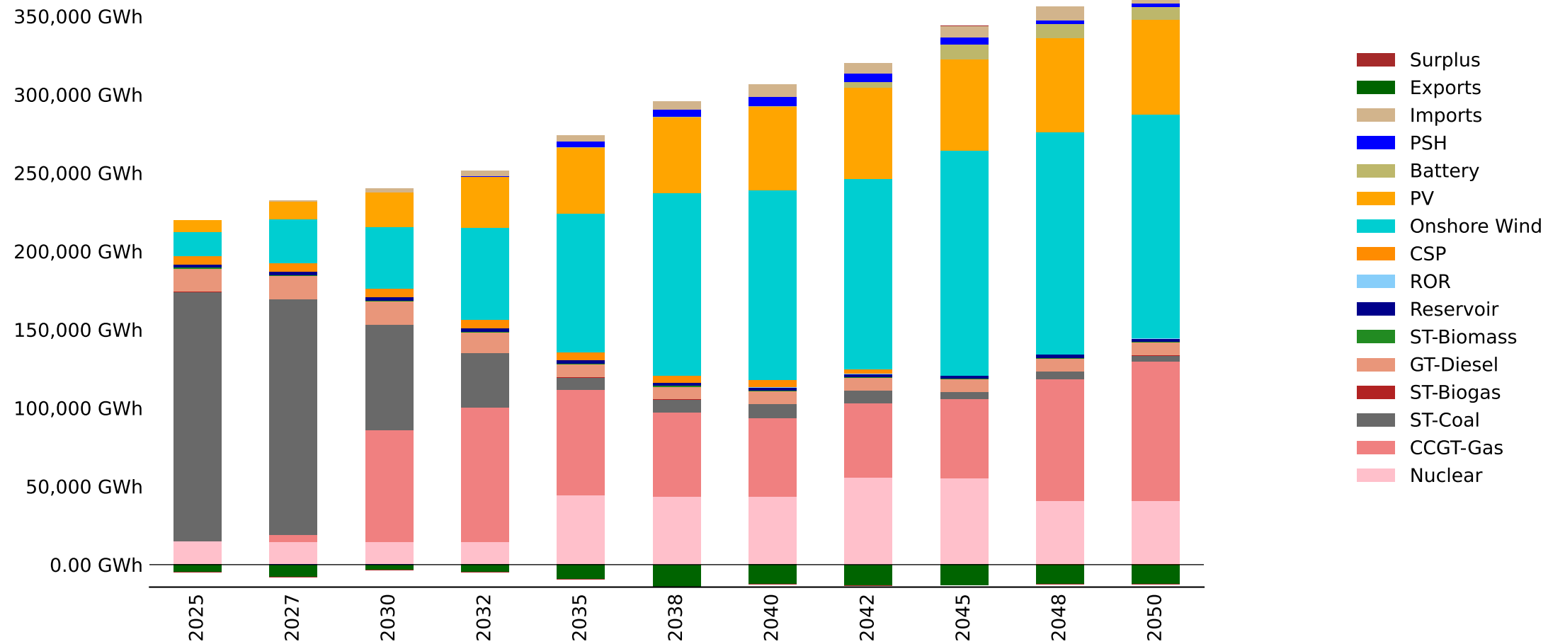
Energy Mix by Fuel - South_Africa - baseline_INGA (GWh)
