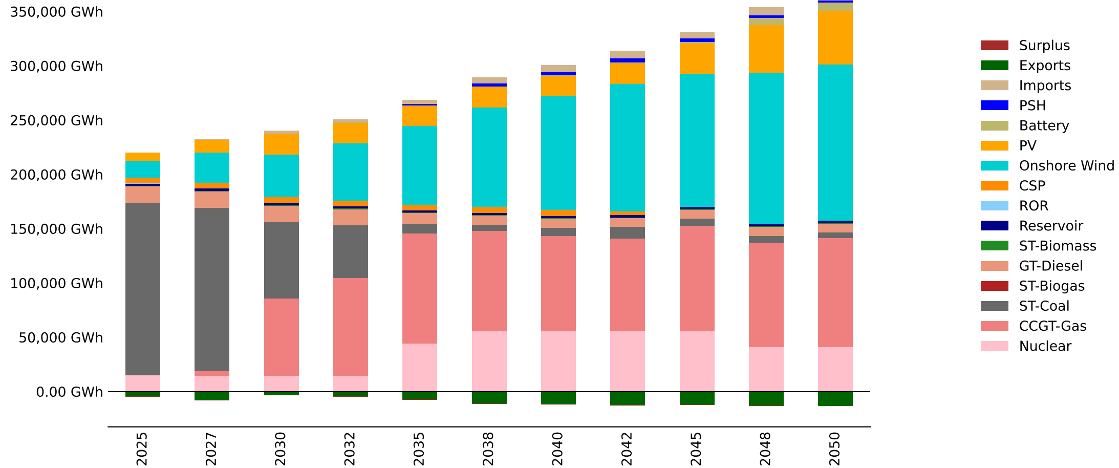
Energy Mix by Fuel - South_Africa - baseline_limexp (GWh)
