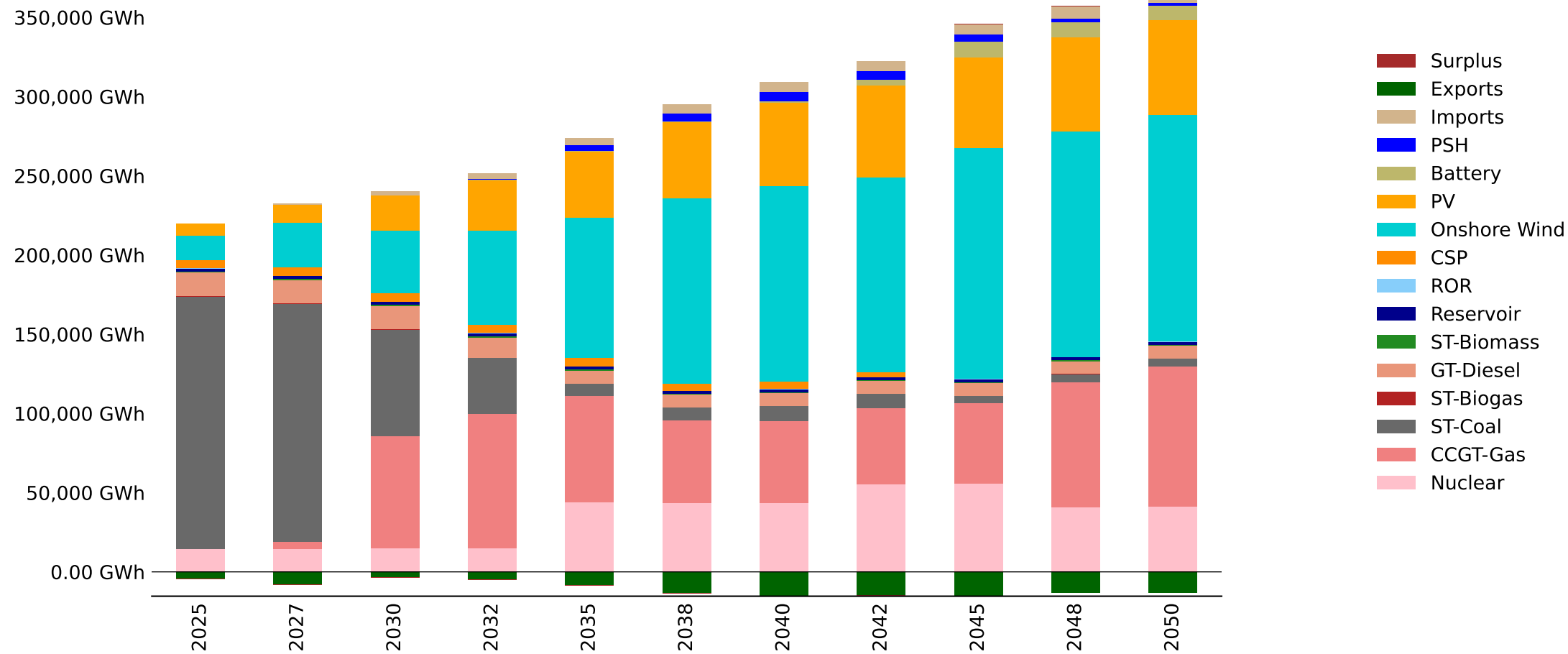
Energy Mix by Fuel - South Africa - baseline noBTKG (GWh)
