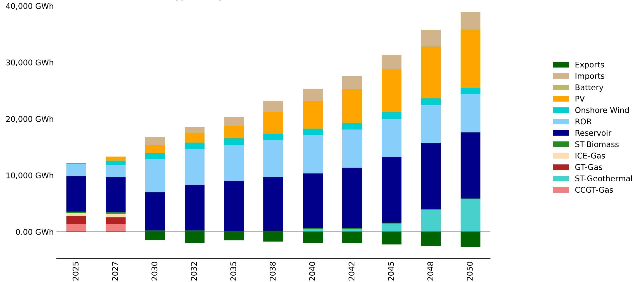
Energy Mix by Fuel - Tanzania - baseline (GWh)
