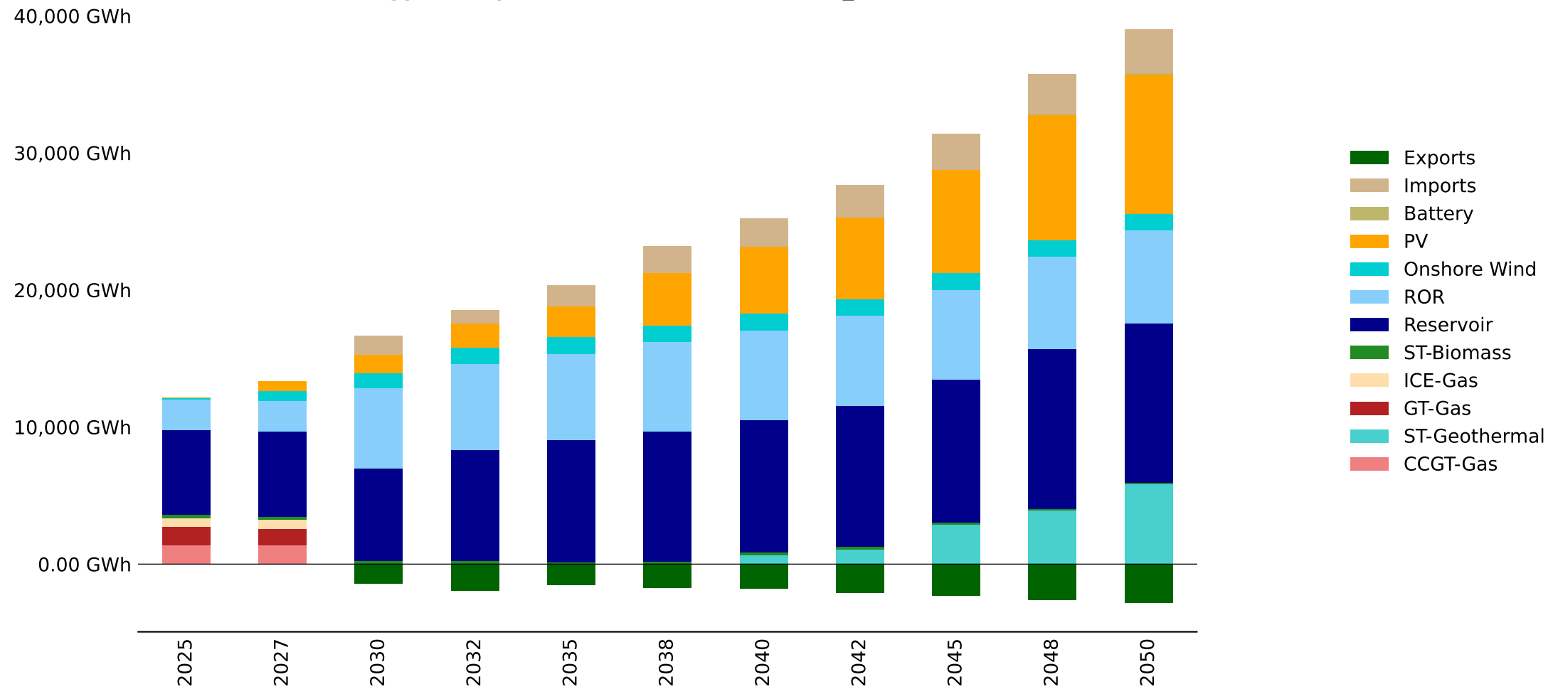
Energy Mix by Fuel - Tanzania - baseline_INGA (GWh)
