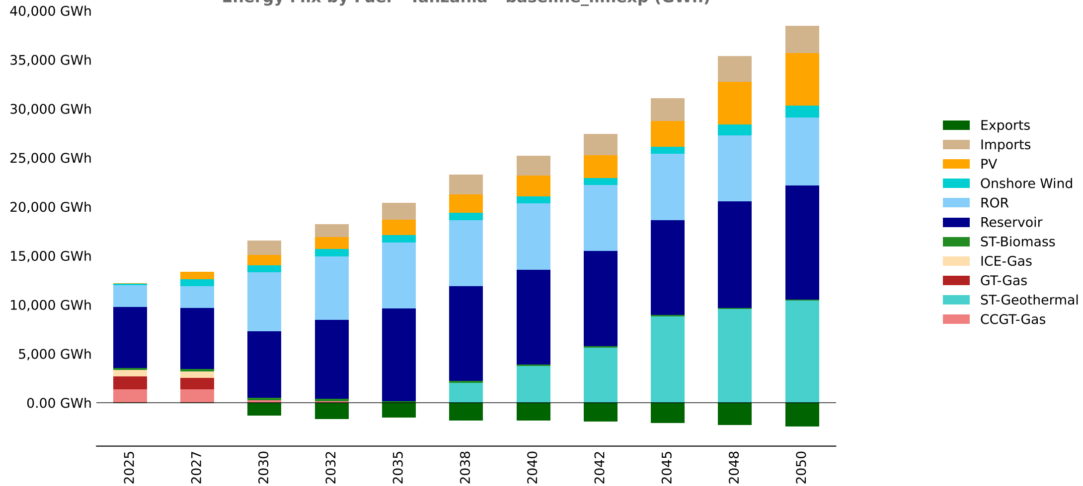
Energy Mix by Fuel - Tanzania - baseline_limexp (GWh)
