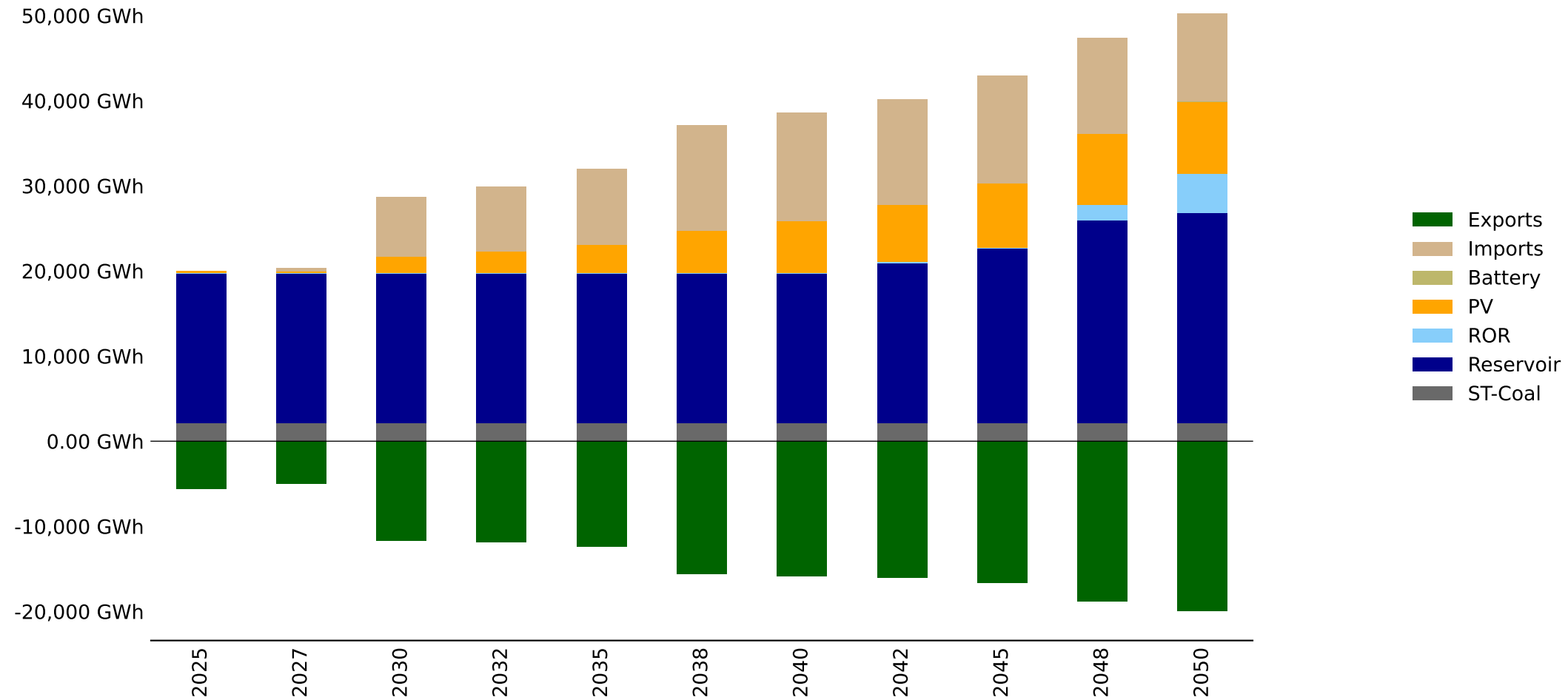
Energy Mix by Fuel - Zambia - baseline (GWh)
