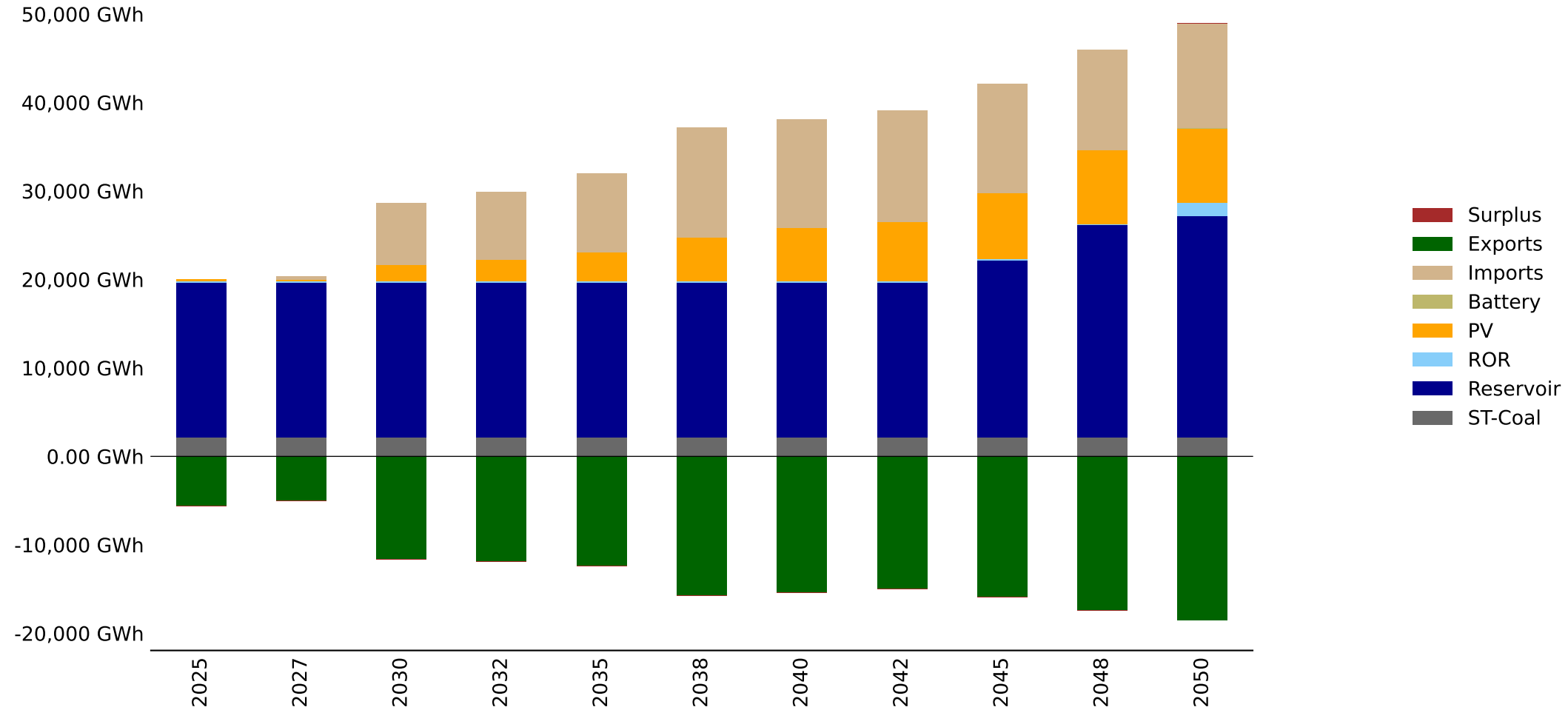
Energy Mix by Fuel - Zambia - baseline_INGA (GWh)
