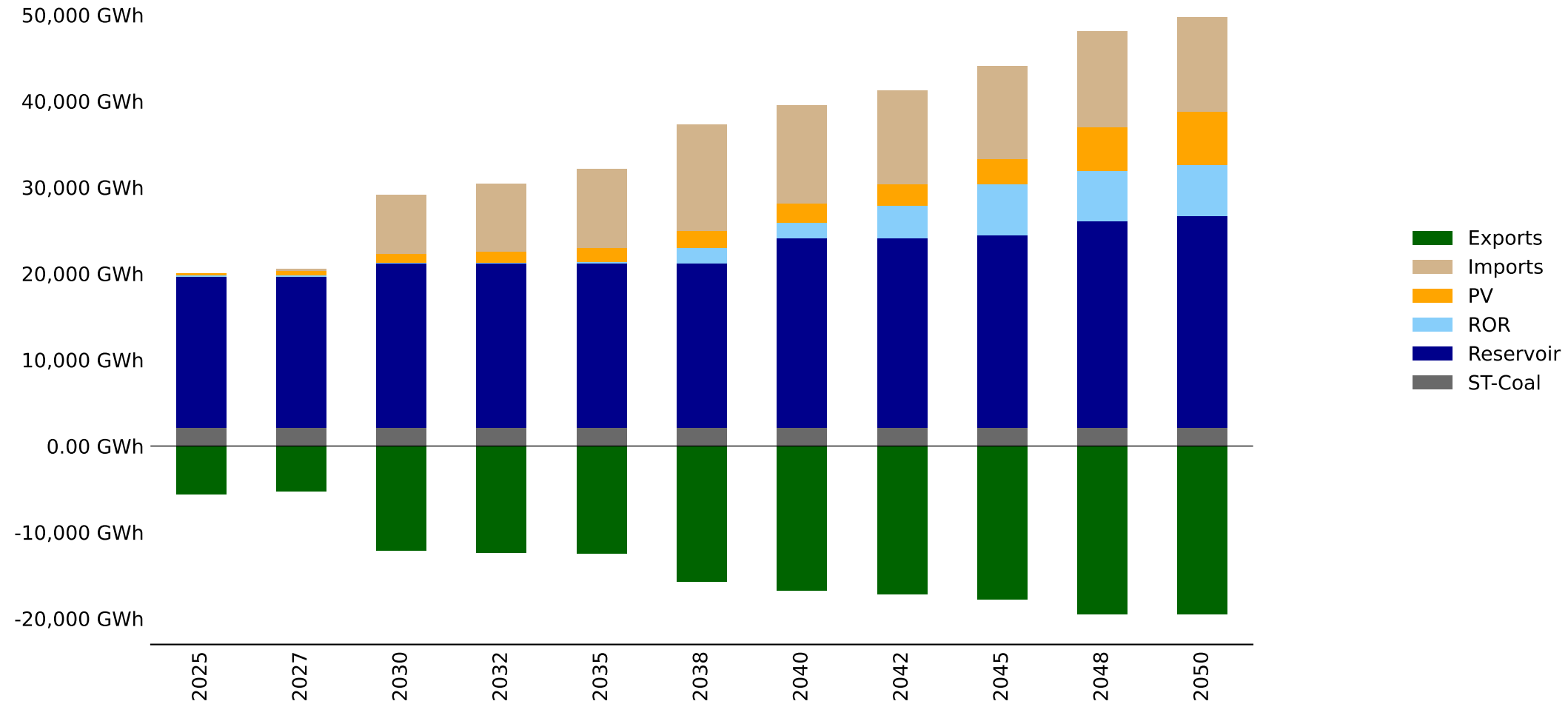
Energy Mix by Fuel - Zambia - baseline_limexp (GWh)
