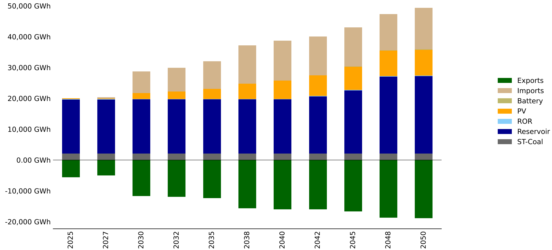
Energy Mix by Fuel - Zambia - baseline_noBTKG (GWh)
