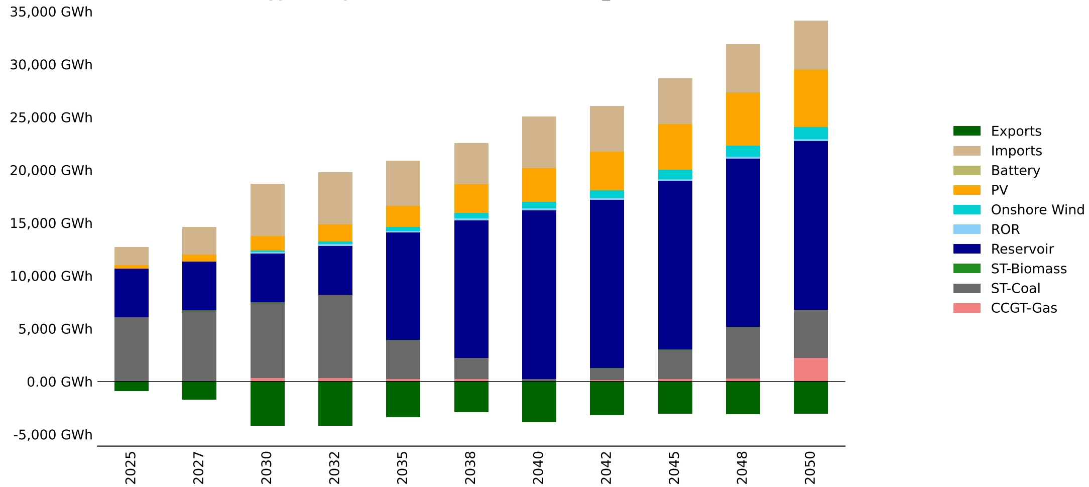
Energy Mix by Fuel - Zimbabwe - baseline_INGA (GWh)
