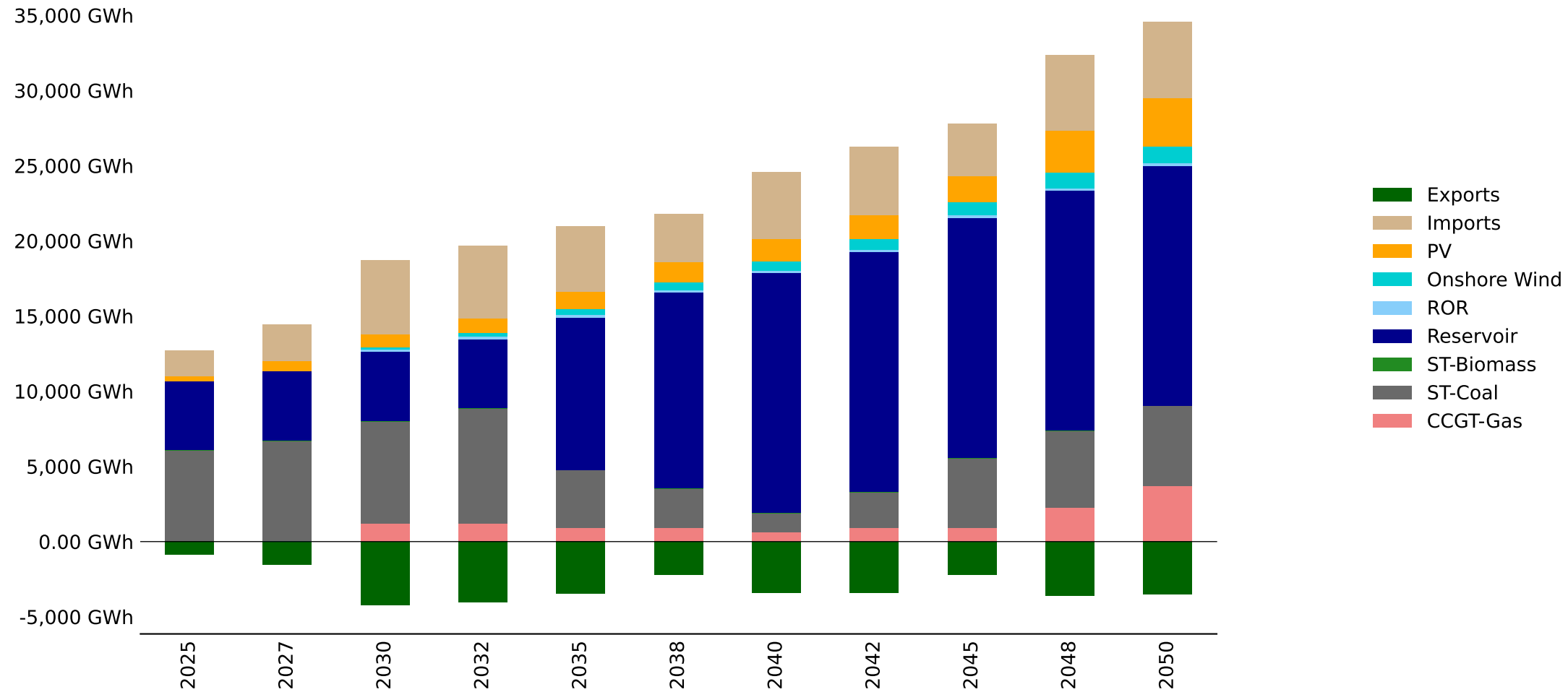
Energy Mix by Fuel - Zimbabwe - baseline_limexp (GWh)
