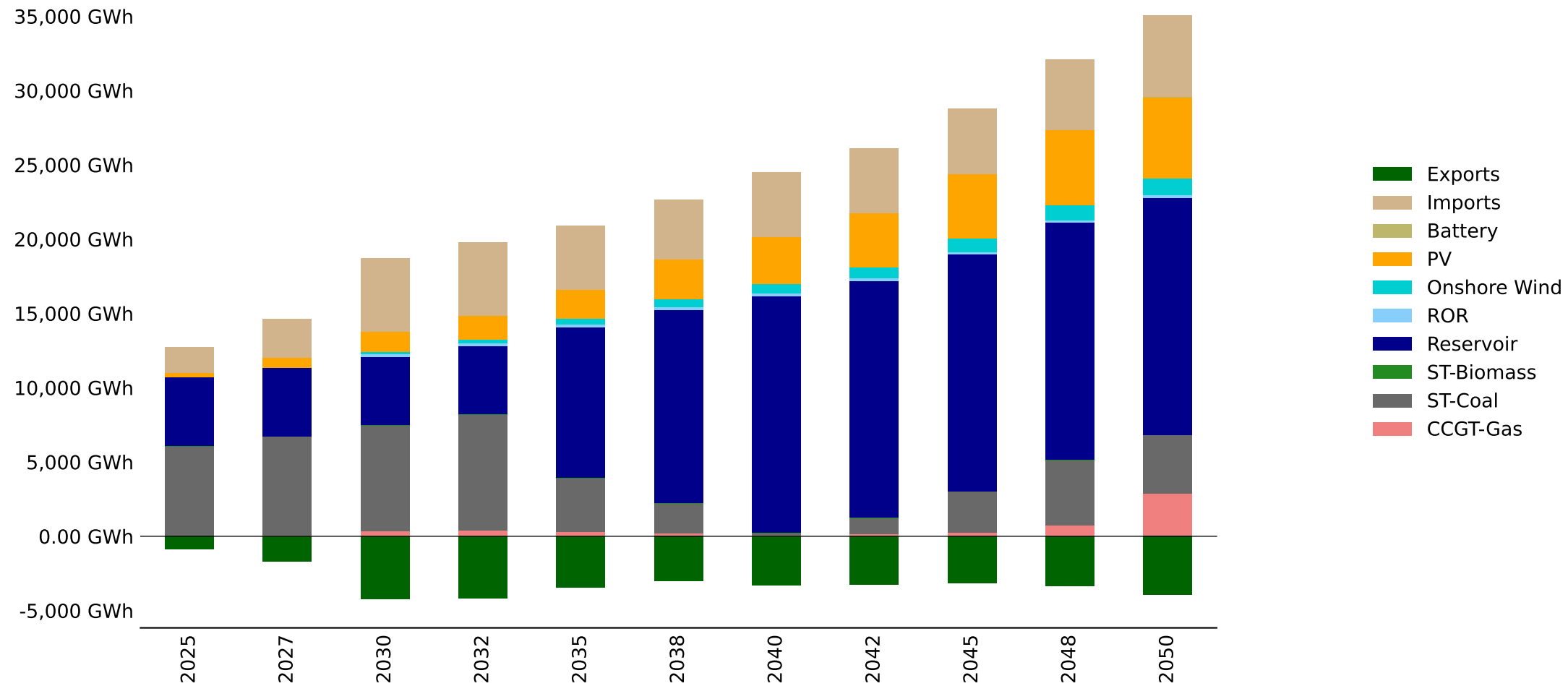
Energy Mix by Fuel - Zimbabwe - baseline_noBTKG (GWh)
