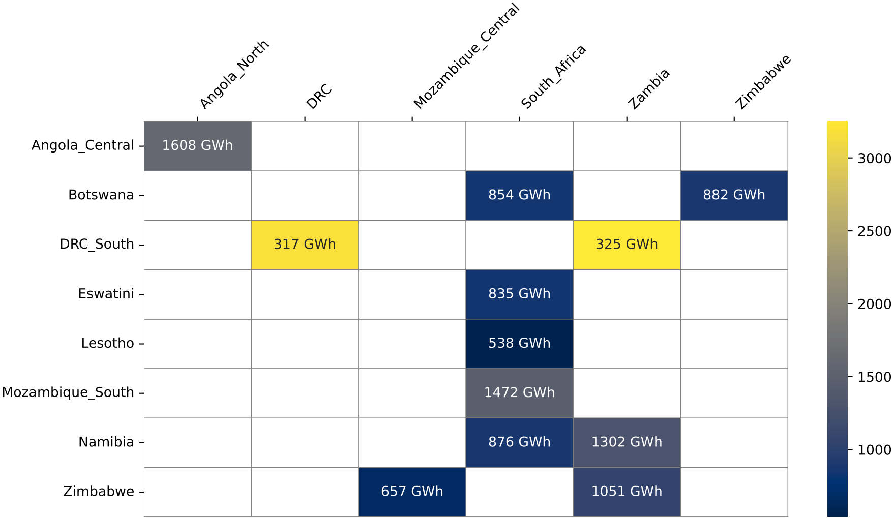
Interconnection Energy Exchange - baseline - 2025 (GWh)
