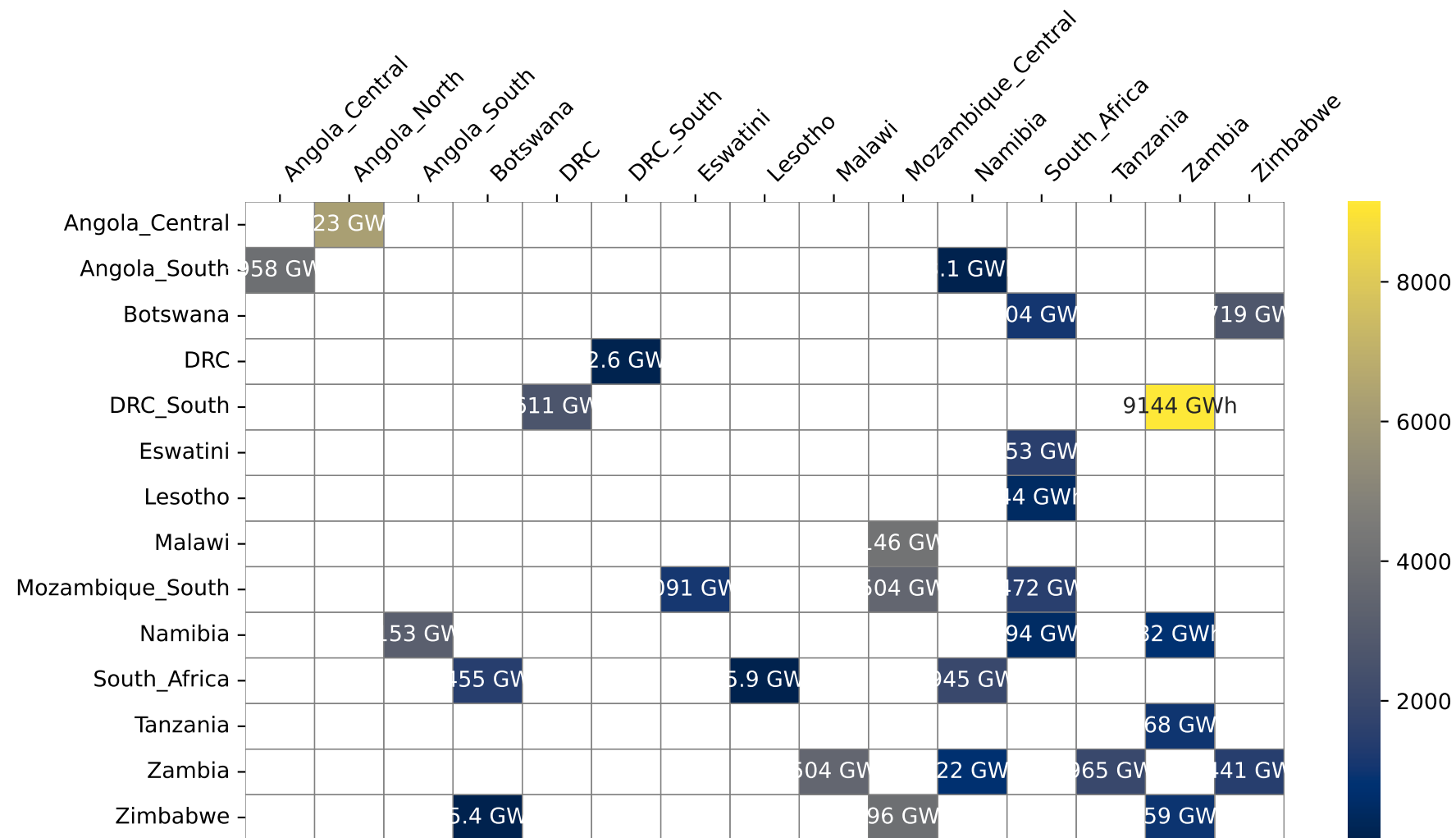
Interconnection Energy Exchange - baseline - 2032 (GWh)
