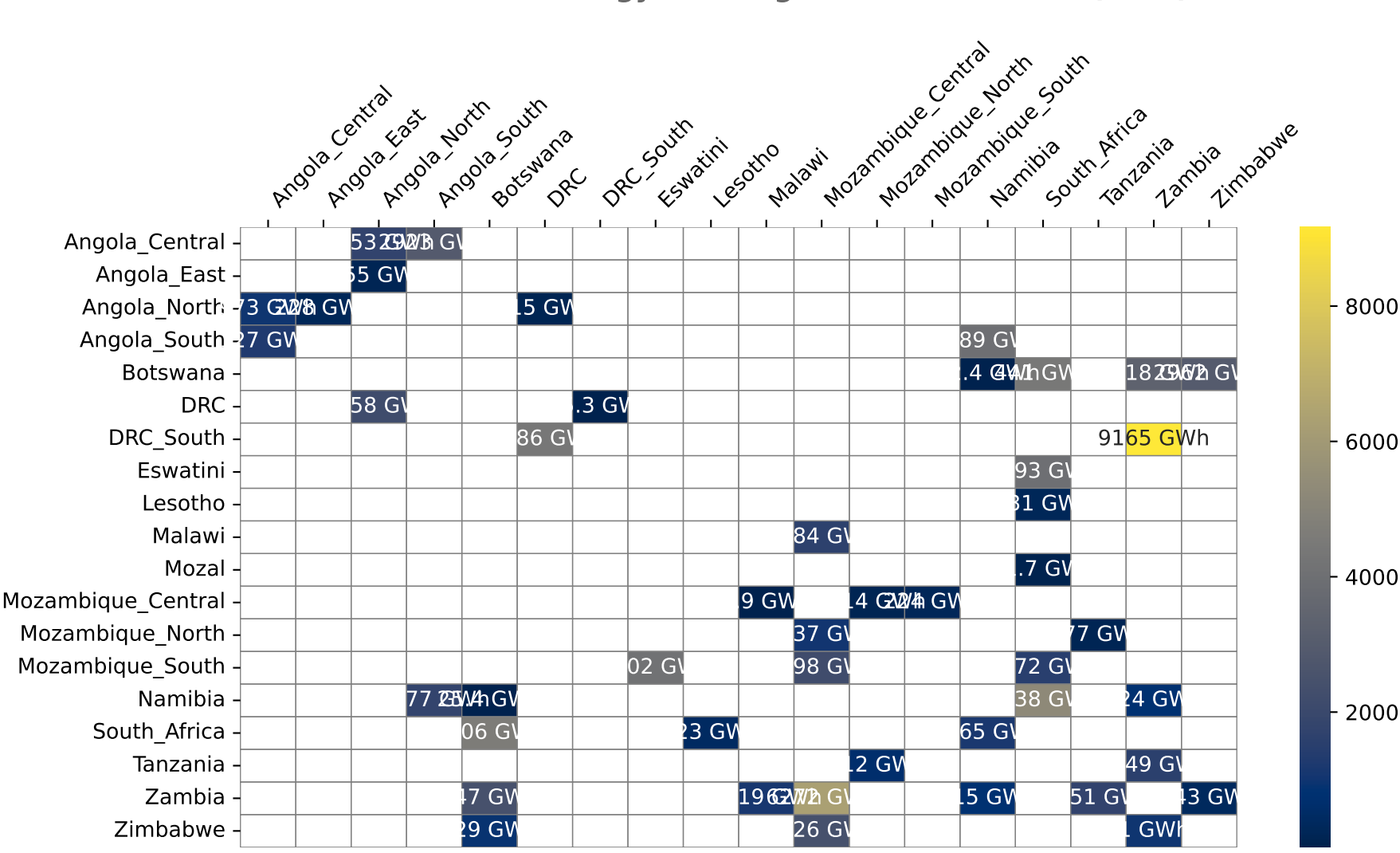
Interconnection Energy Exchange - baseline - 2040 (GWh)
