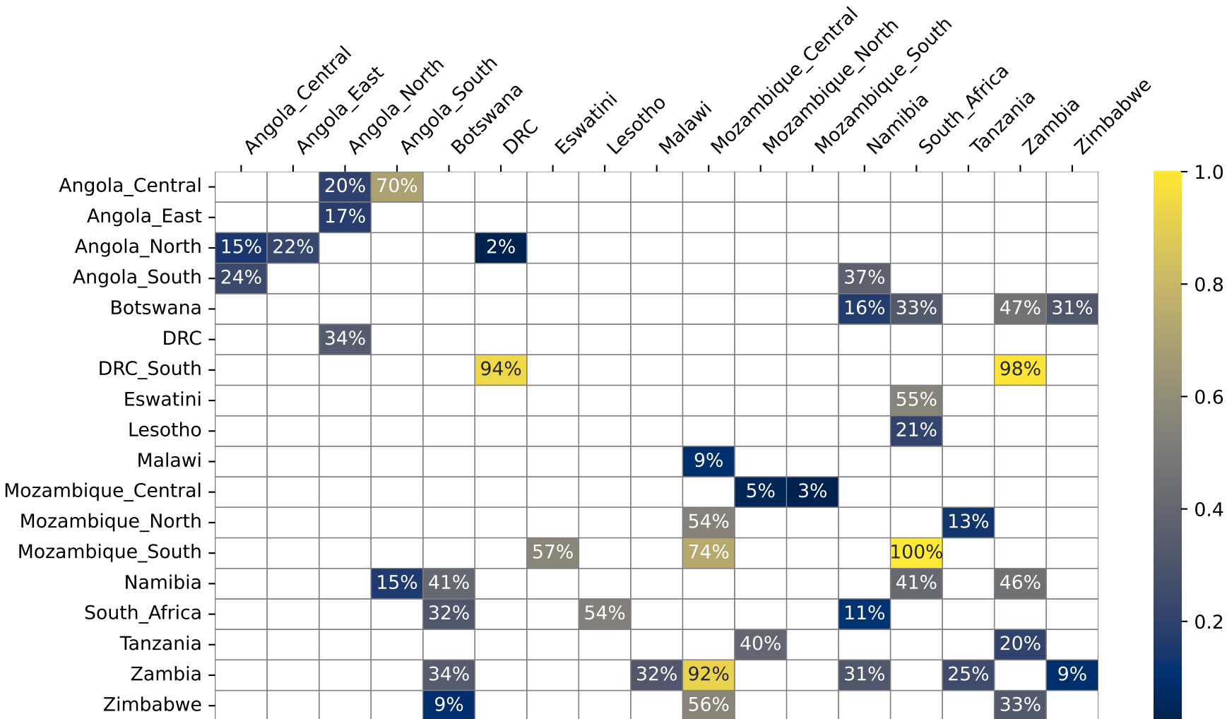
Interconnection Utilization - baseline - 2042 (%)
