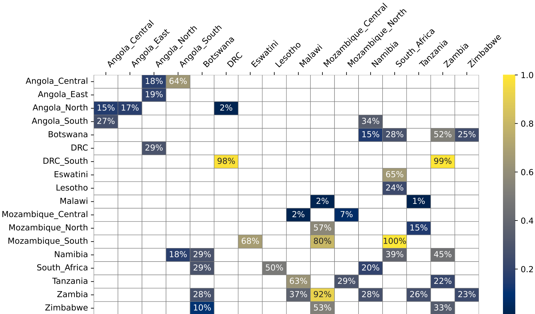
Interconnection Utilization - baseline - 2045 (%)
