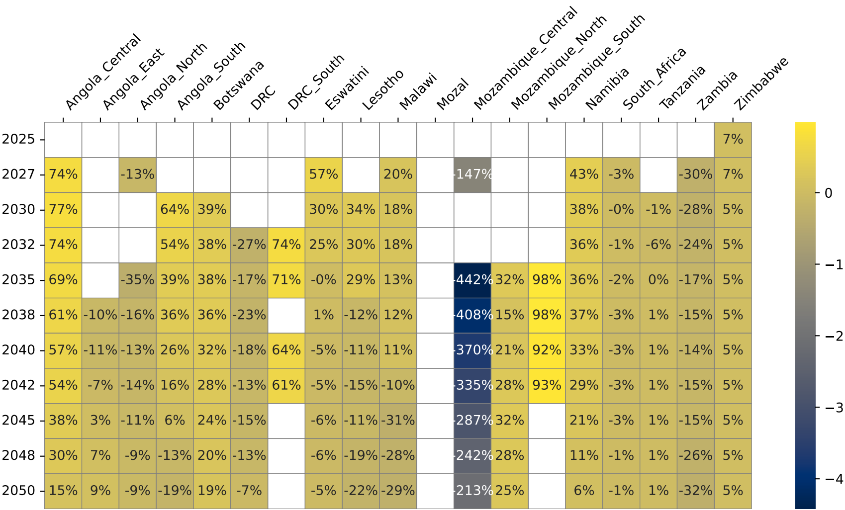
Net Imports by Zone over Time - baseline [% of energy demand]
