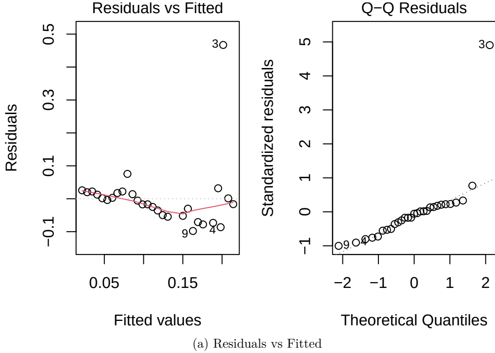
Figure 6: Residual plots for HHI model
