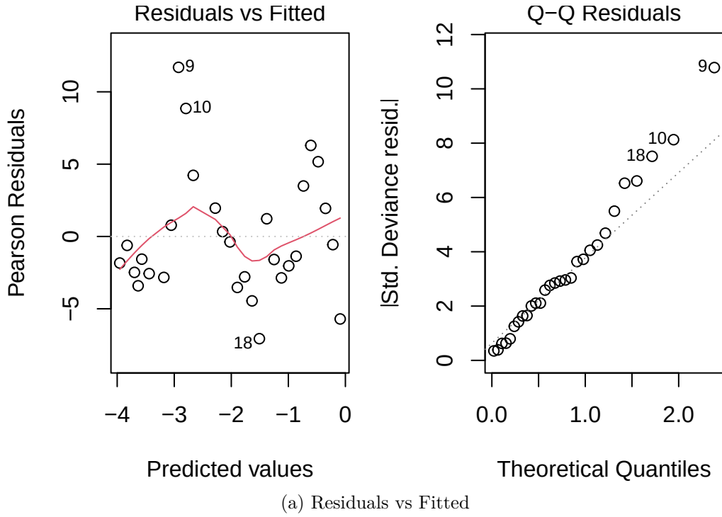
Figure 4: Residual plots for female representation model
