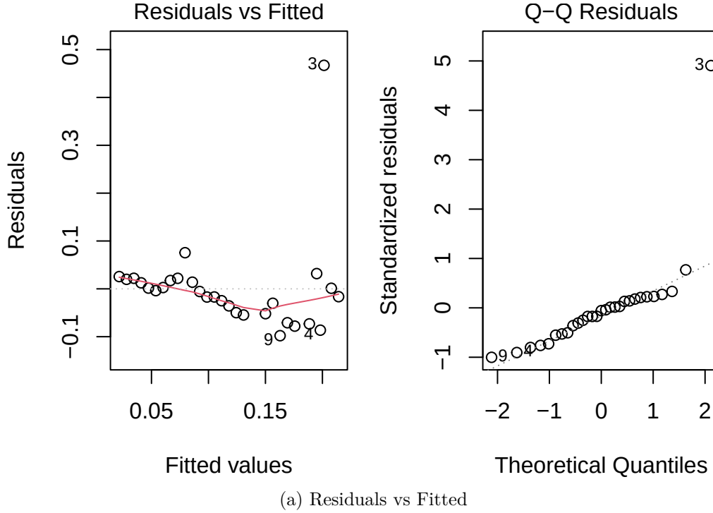
Figure 6: Residual plots for HHI model
