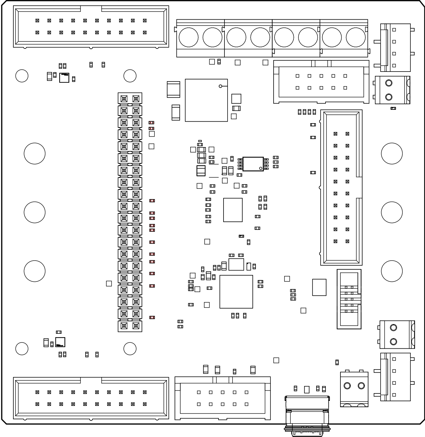
View from Top side (Scale 2:1)
