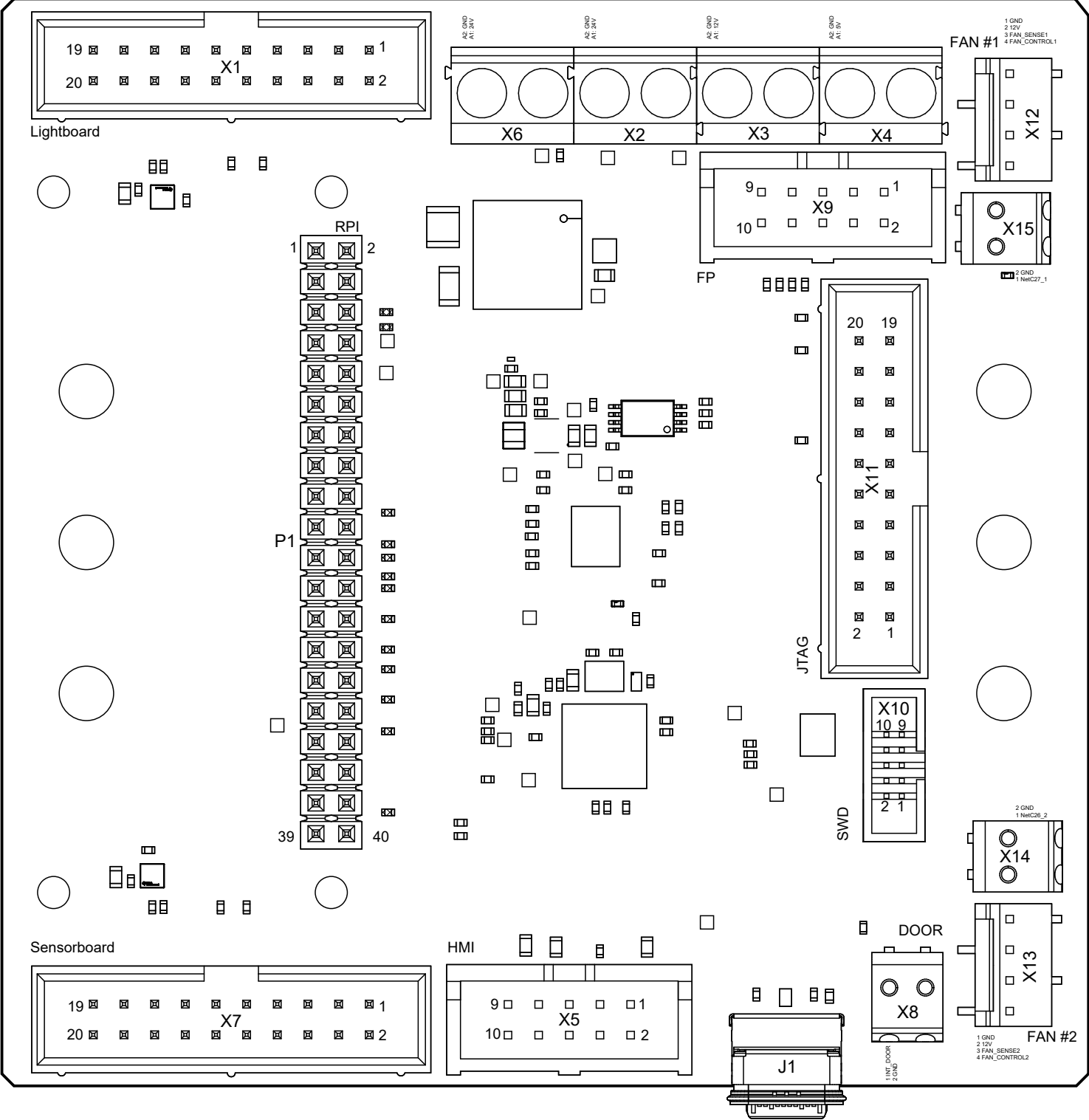
View from Top side (Scale 2.1631:1)
