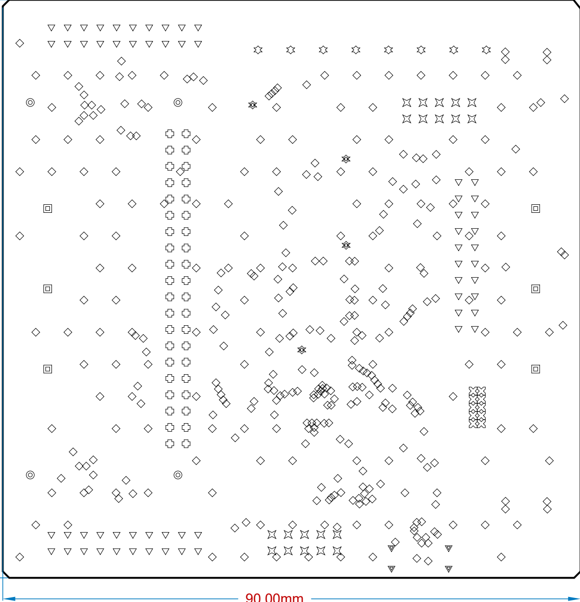
Drill Drawing View (Scale 1.7:1)
