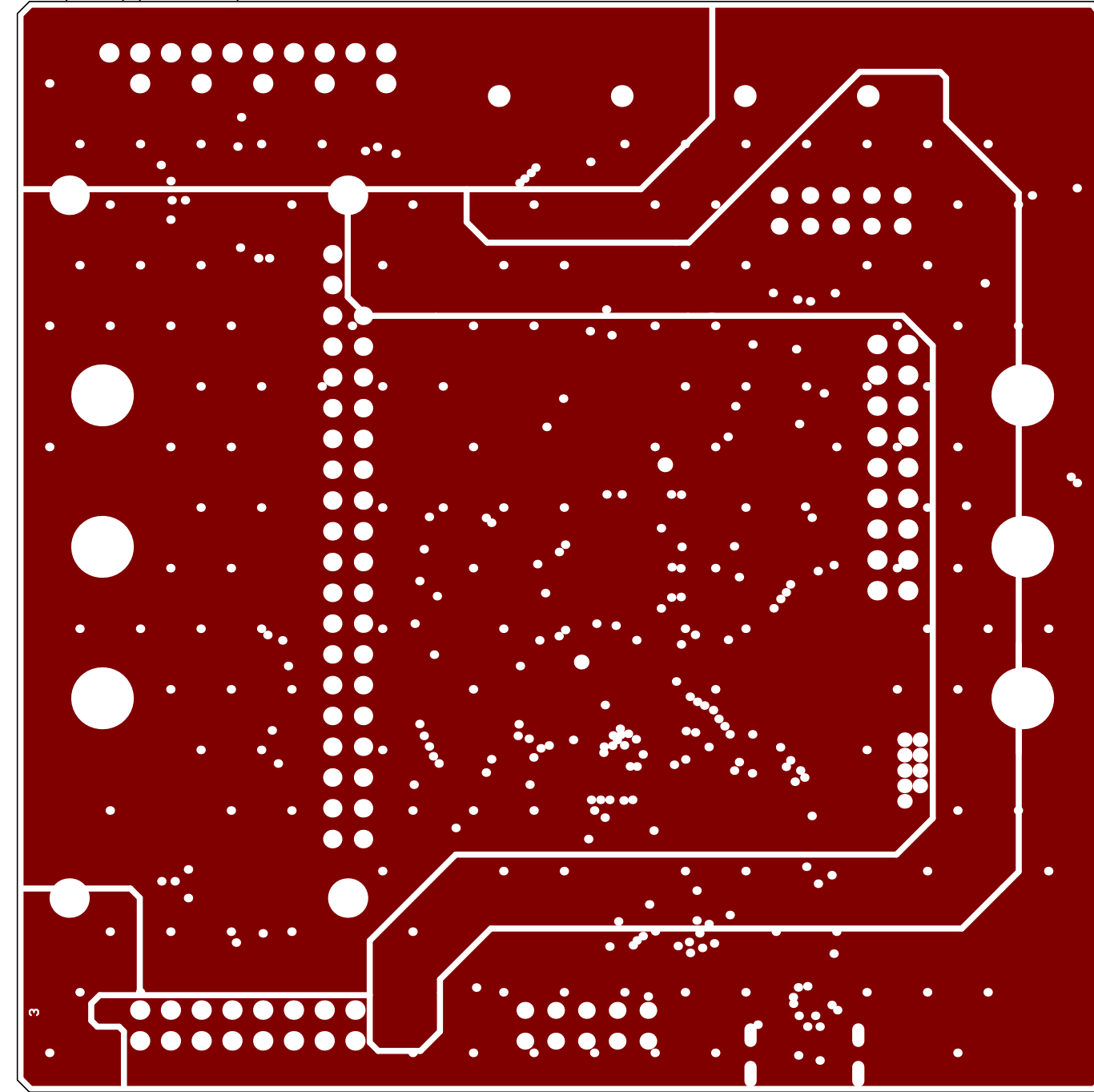
Int2 (PWR) (Scale 2:1)
