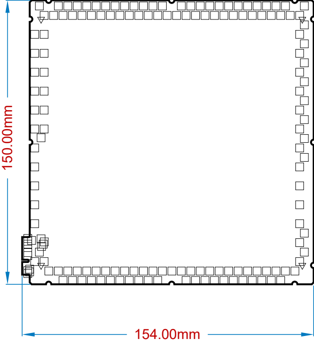
Drill Drawing View (Scale 1:2)
