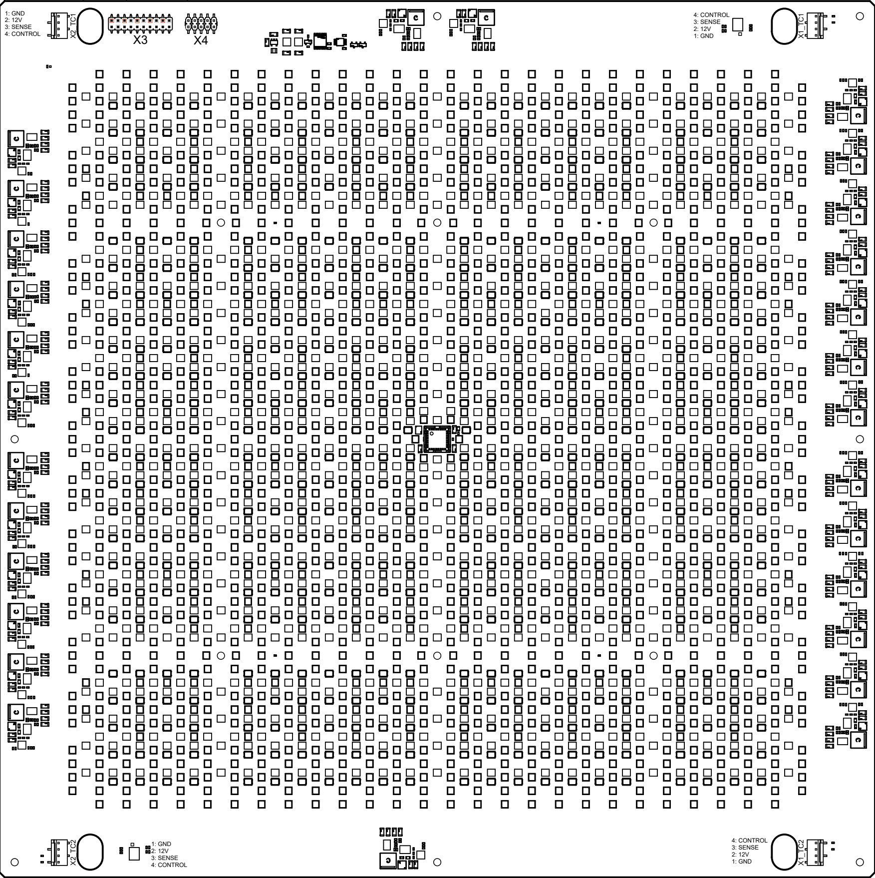
View from Top side (Scale 2:3)
