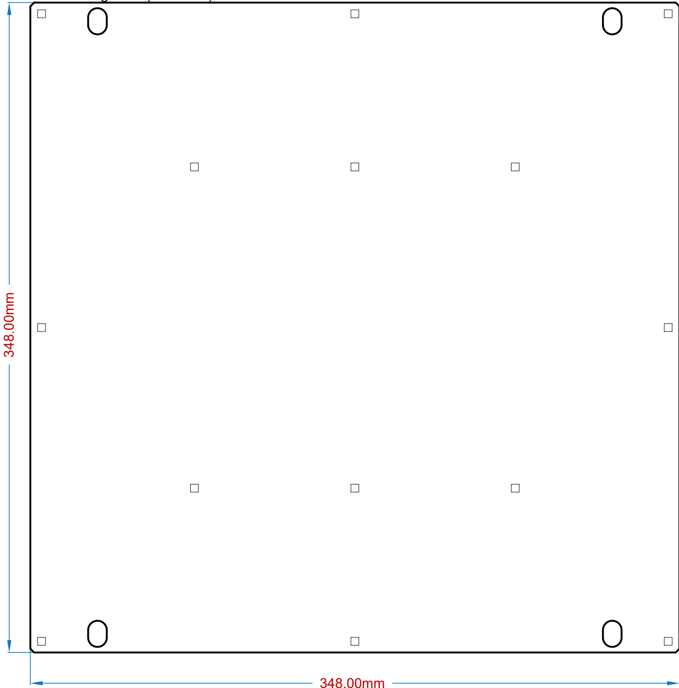
Drill Drawing View (Scale 1:2)
